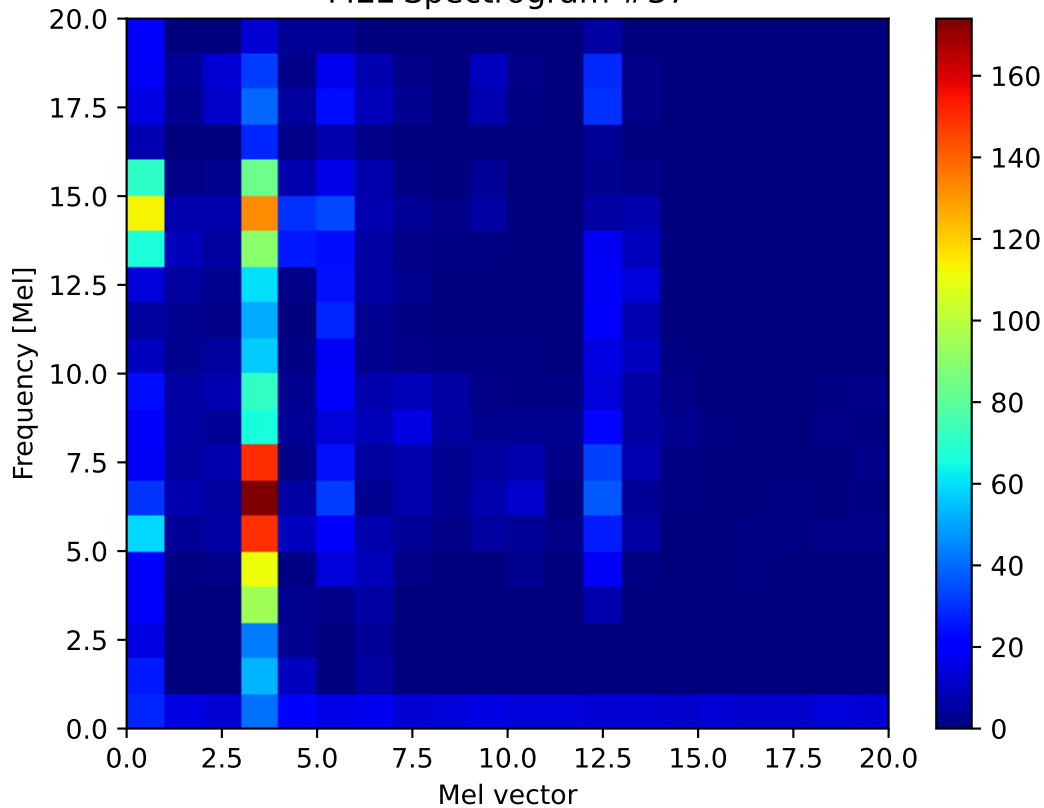
MEL Spectrogram #37
